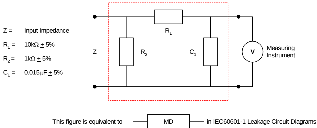
Figure 2-8: Required Test Load
