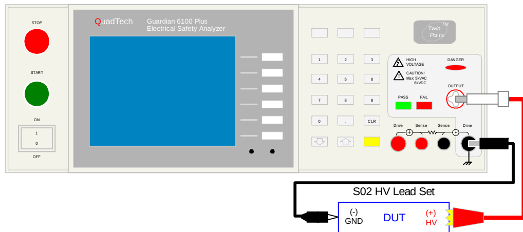
Figure COI-3: S02 Cable Connection To Device Under Test
