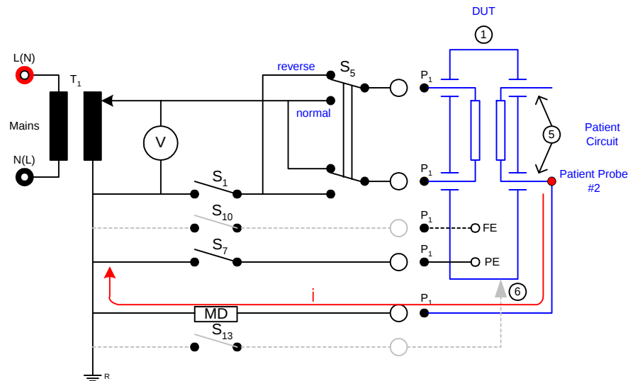
Figure 2-14a: Patient Leakage – Applied Part to Ground (Figure 14 of 60601-1 © IEC 2000)
