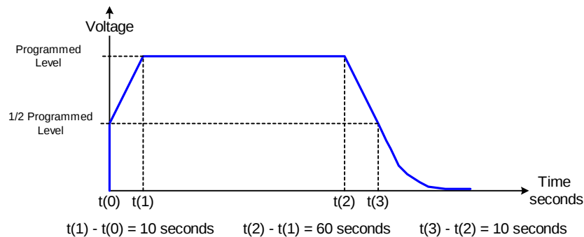
Figure 2-20: 1/2 Programmed Test Voltage
