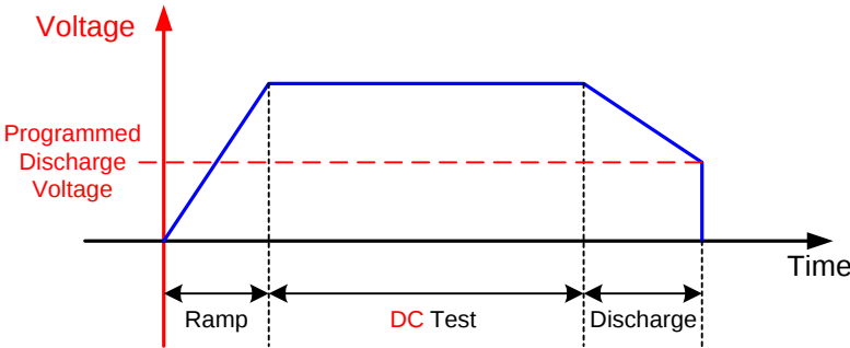
Figure 2-3: Discharge Voltage
